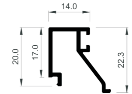
COR-3811 Bead 14 mm
