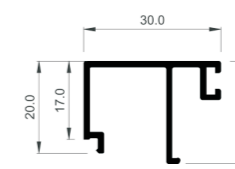
COR-3810 Bead 30 mm
