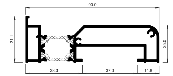
COR-3836 Subcill 90 mm
