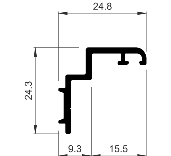
COR-3746 Swing door rebate
