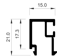
COR-3781 15 mm glazing bead
