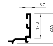
COR-3783 3,7 mm glazing bead
