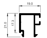
COR-3780 19 mm bead
