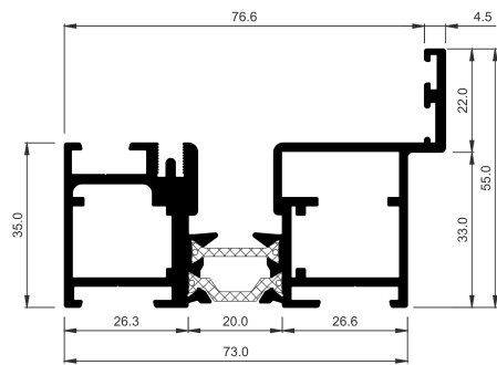
COR-3730 Frame with inox rail
