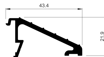
COR-3792 20 mm ramp for threshold
