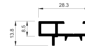
COR-3744 Half roller adapter
