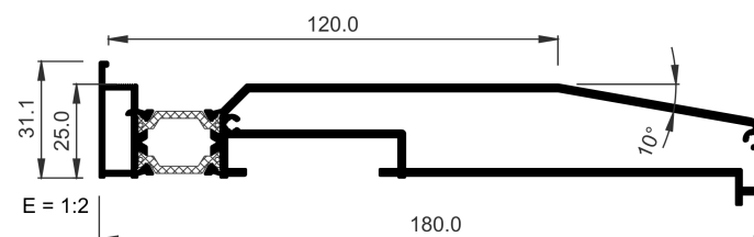
COR-3837 Subcill 180 mm
