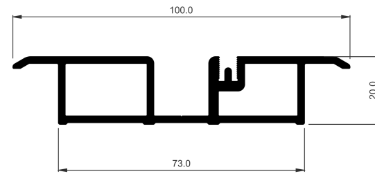
COR-3790 Threshold
