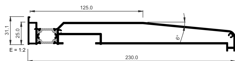
COR-3838 Subcill 230 mm
