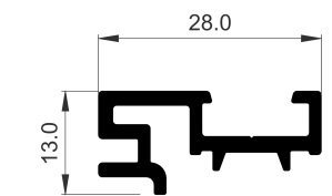
COR-3742 Lock keep adaptor
