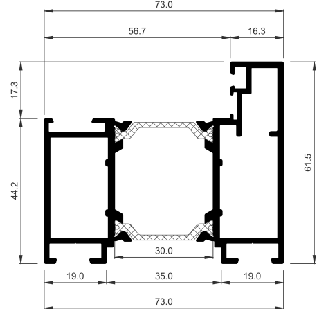
COR-3720 Standard sash
