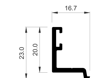
COR-3792 20 mm ramp for threshold
