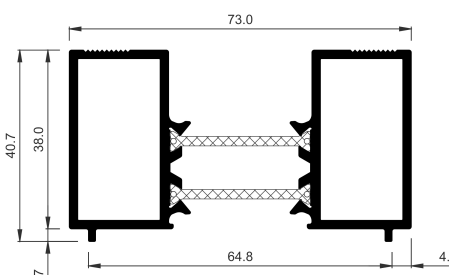
COR-3795 Frame supplement
