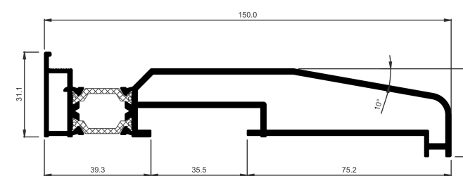
COR-3735 150 mm drainage subcill
