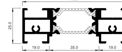
COR-3741 Sliding post
