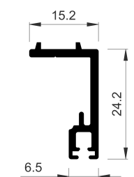
COR-3725 Sash extension
