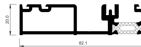
COR-3791 20 mm threshold with thermal break
