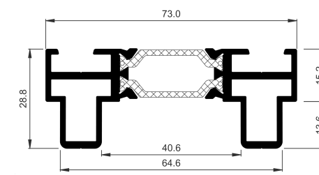
COR-3740 Adjustable jamb
