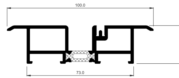
COR-3789 Threshold with thermal break
