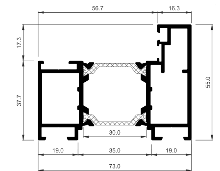
COR-3721 55 mm sash
