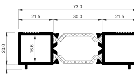
COR-3796 Frame supplement 20 mm
