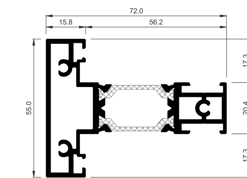
COR-3770 Sash transom
