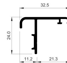
COR-3745 Swing door rebate
