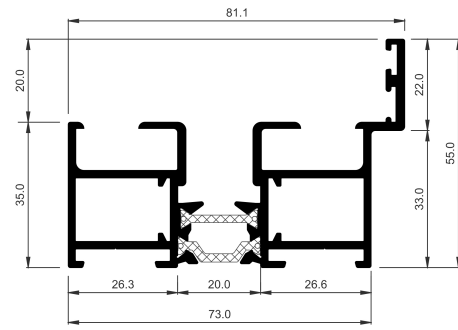
COR-3731 Lateral frame
